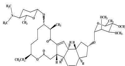
Spinosyn A (C 41 H 65 NO 10 ) MW 731.461
